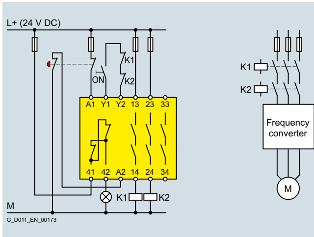
Conventional wiring
