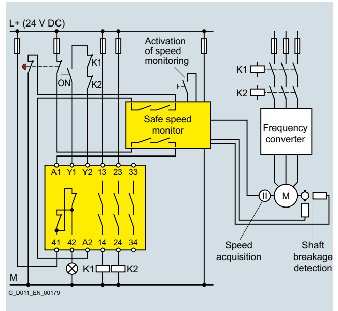
Conventional wiring
